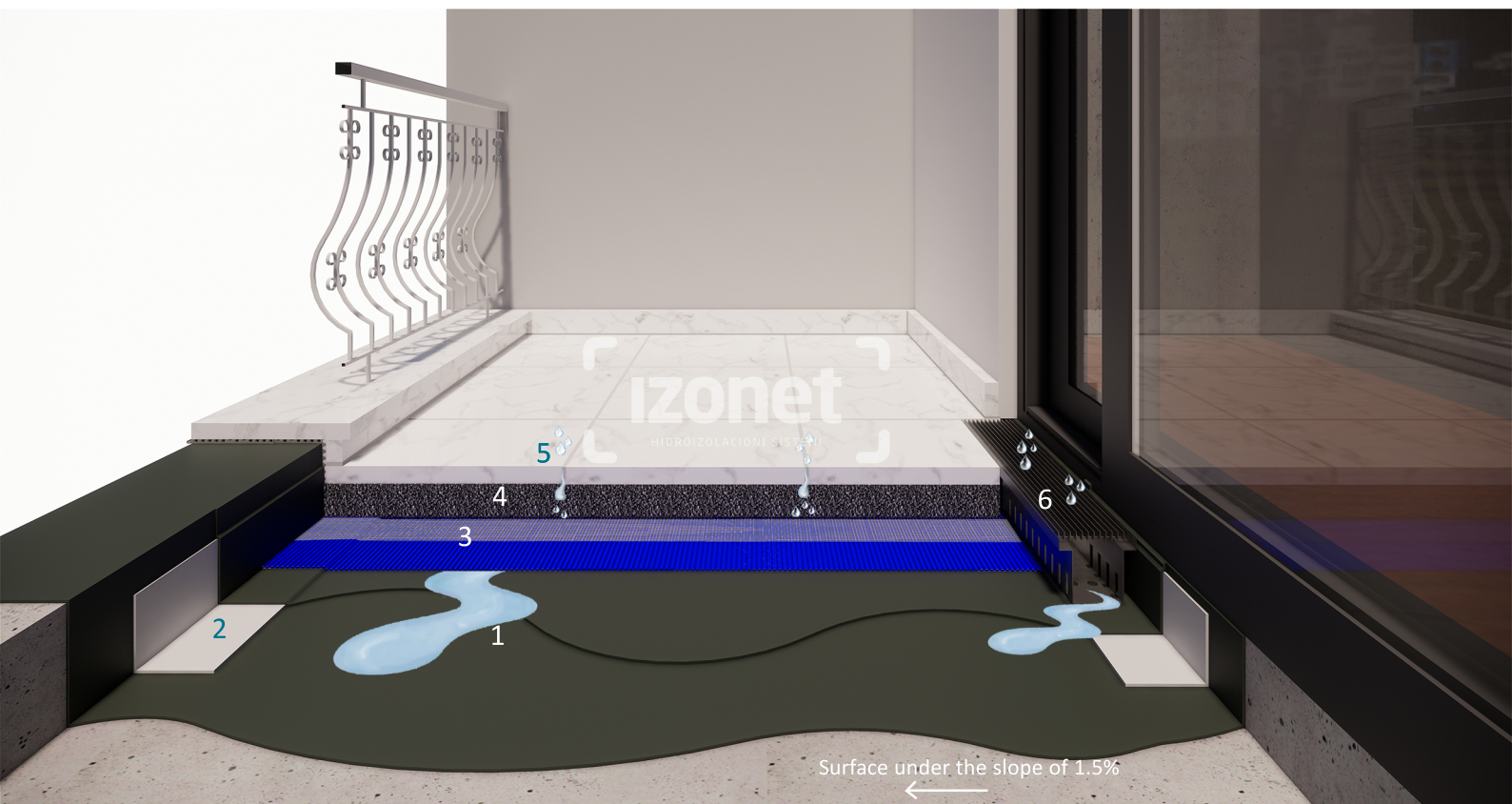
1. ARDEX 8+9 waterproof layer 2. ARDEX SK 12 tape 3. AQUADRAIN® EK drainage layer 4. ARDEX A10 + ARDEX QUARKIES ME granulation 3.0 - 5.6 mm 5. stone/ceramic paving 6. AQUADRAIN FLEX line drain
